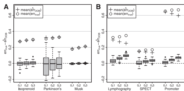
Fig. 4. Difference of true imputation error err_{true} and OOB imputation error estimate \widehat{err}_{OOB} for the continuous datasets (A) and the categorical datasets (B) and three different amounts of missing values, i.e. 0.1, 0.2 and 0.3. In each case, the average err_{true} (circle) and the average \widehat{err}_{OOB} (plus) over all simulations is given.
